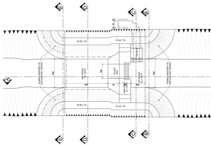
PLAN SCALE 1:25 MTS
